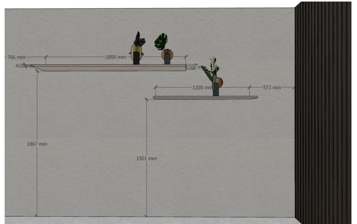
WALL SHELF
